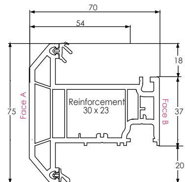
546856 586855 (FOILED) CASEMENT 'I' SASH 75MM (5 CHAMBER)
