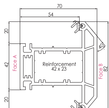
546475 576026 (FOILED) LARGE TRANSOM/ MULLION 'T' 82MM
