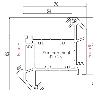
546465 576046 (FOILED) LARGE TRANSOM/ MULLION 'Z' 82MM
