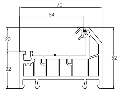
546845 CASEMENT SLIM OUTER FRAME 52MM (6 CHAMBER)
