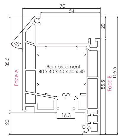
546625 576625 (FOILED) DOOR 'Z' SASH 105.5MM
