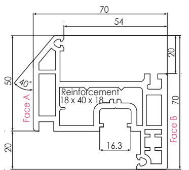
546776 576776 (FOILED) TILT/TURN SASH 70MM
