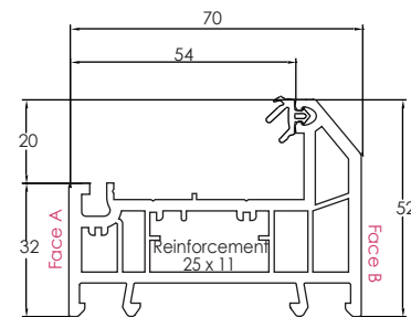
586815 (FOILED) CASEMENT SLIM OUTER FRAME 52MM (5 CHAMBER)
