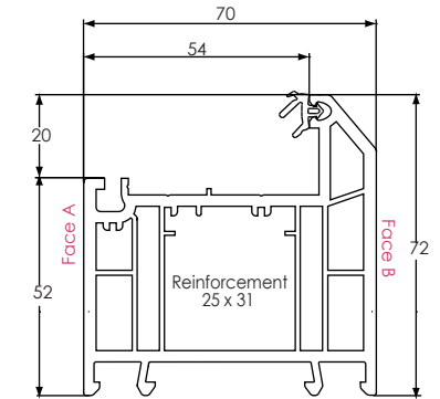
586835 (FOILED) CASEMENT LARGE OUTER FRAME 72MM (5 CHAMBER)
