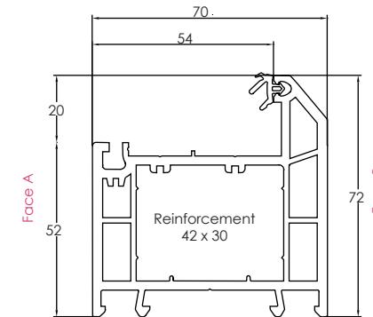
546185 576365 (FOILED) CASEMENT LARGE OUTER FRAME 72MM (3 CHAMBER)
