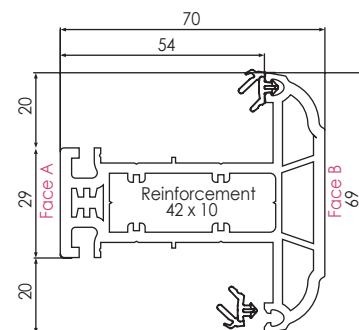
546665 576665 (FOILED) SLIM SCULPTURED TRANSOM/MULLION 'T' 69MM
