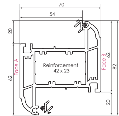
546755 576755 (FOILED) LARGE SCULPTURED TRANSOM/MULLION 'Z' 82MM
