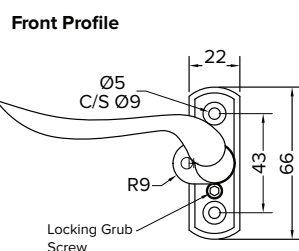
Regent Window Espag Window Handle - REG020
