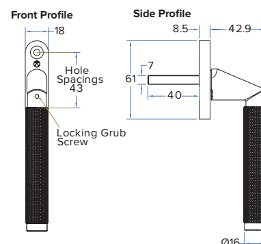
Newton Knurled Inline Window Espag Handle - NTN340
