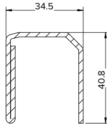
357832 REINFORCEMENT 34.1 X 40.8 X 2MM
