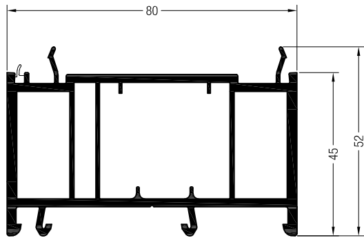
538045 568045 (Foiled) Reinforcement 23 x 28 45MM FRAME EXTENSION
