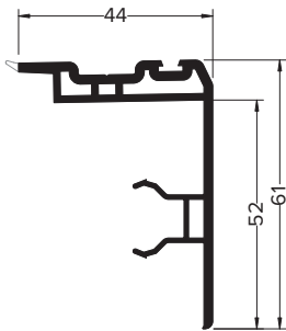
575506 595606 (Foiled) INTERLOCK
