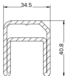
357833 REINFORCEMENT 34.1 X 40.8 X 2.5MM
