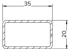
357836 REINFORCEMENT 35 X 20 X 1.5MM
