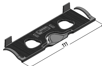
375310 GLAZING PACKER
