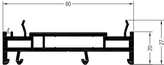
538025 568025 (Foiled) Reinforcement 35 x 6 20MM FRAME EXTENSION
