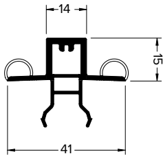
575507 3/4 PANE SEAL
