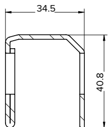
361488 REINFORCEMENT 34.1 X 40.8 X 2MM
